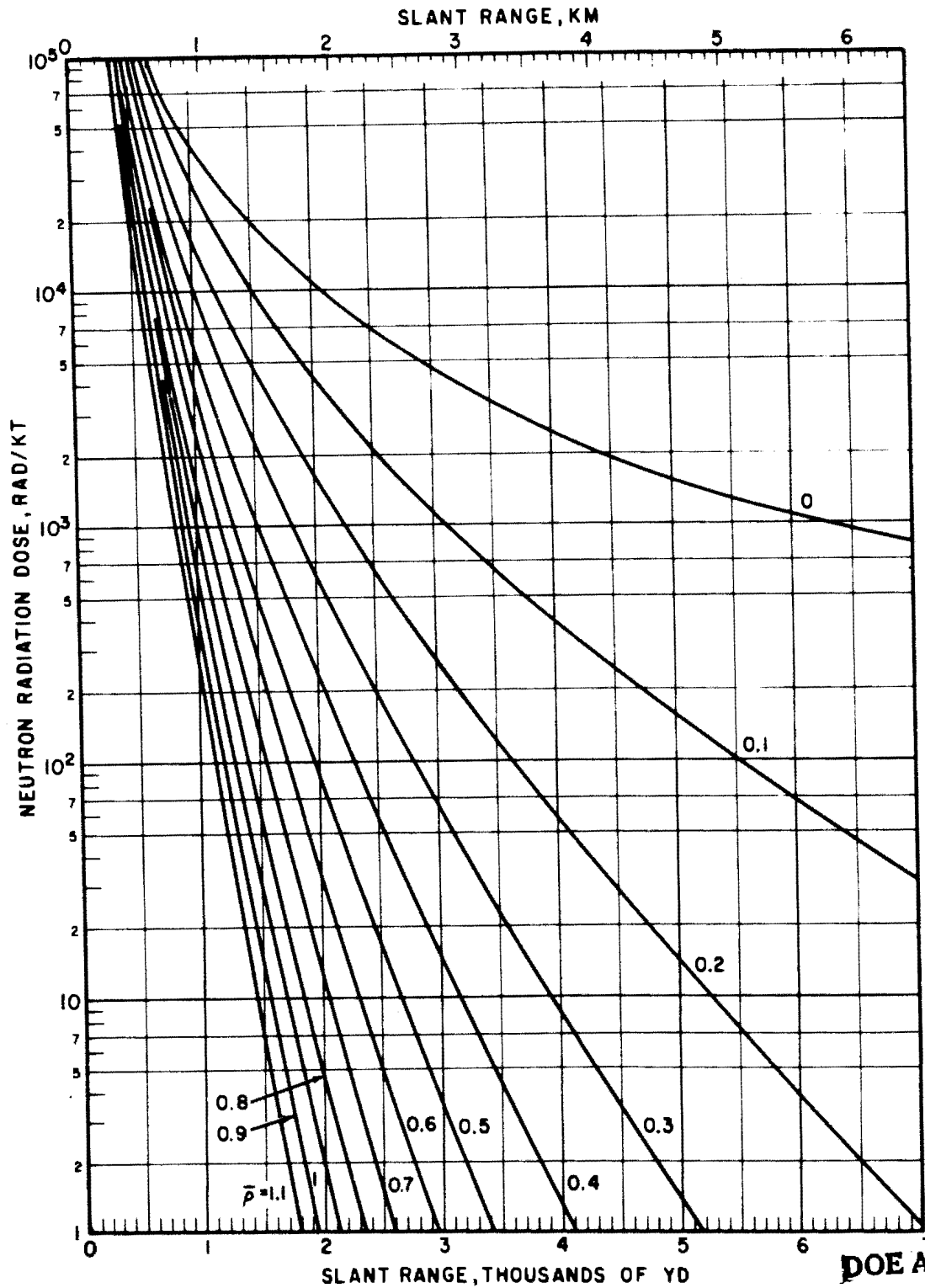
Figure 4-19. Neutron Radiation Dose vs. Slant Range for Various Average Relative Air Densities, 1-kt (High Flux Fission) Air Burst-Surface Target
